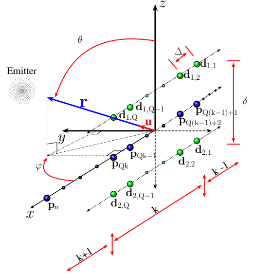
Fig. 1: Synthetic aperture for Q samples and K snapshots.
