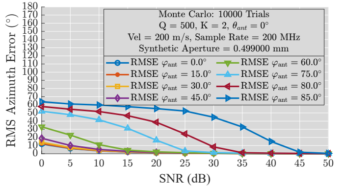
Fig. 4: RMS azimuth error as a function of \varphi_{\text{ant}} .
